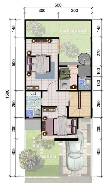
Denah Lantai 2
